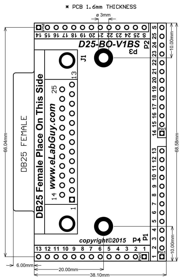
D25-BO-V1BS PCB outline Drawing
